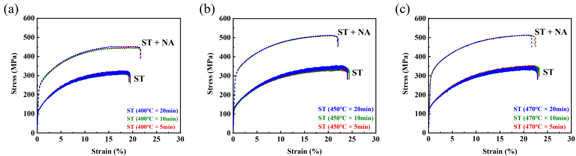
Fig. S1. Effect of natural-aging on tensile properties after solution treatment (a) 400 °C, (b) 450 °C, (c) 470 °C
