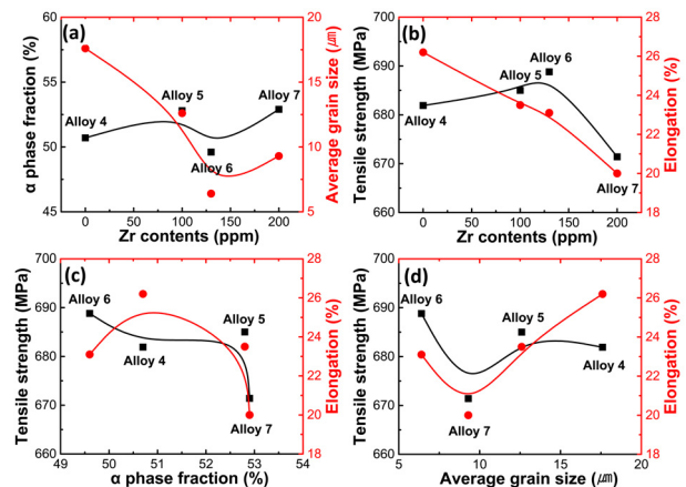
Fig. 7. (a) Measured \alpha phase fraction and average grain size of the Ni-Al-Bronze alloys with different zirconium contents. Tensile strength and elongation of Ni-Al-Bronze alloys with different (b) zirconium contents, (c) \alpha phase fraction and (d) average grain size.
